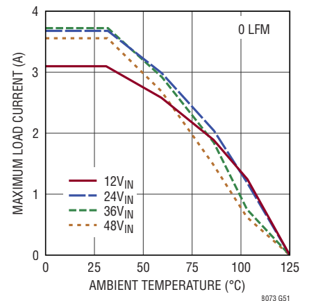
Derating, V_{OUT} = -5\text{V} , BIAS = 0V, DC2389A Demo Board
