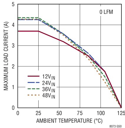
Derating, V_{OUT} = -3.3\text{V} , BIAS = 0V, DC2389A Demo Board
