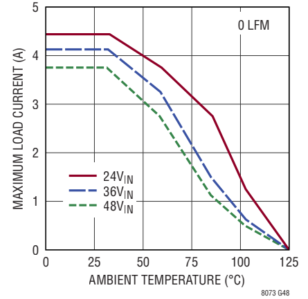
Derating, V_{OUT} = 12\text{V} , BIAS = 5V, DC2389A Demo Board
