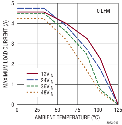
Derating, V_{OUT} = 8\text{V} , BIAS = 5V, DC2389A Demo Board
