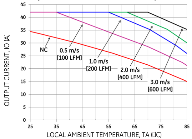
Figure 21. Output Current Derating for the Base plate QSVW042A0B-H +0.5" Heat sink in the Longitudinal Orientation; Airflow Direction from Vout to Vin; Vin = 48V.
