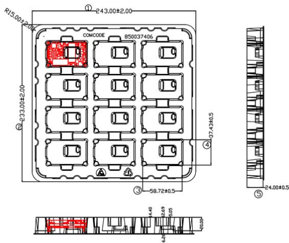
Base Plate Module Tray
