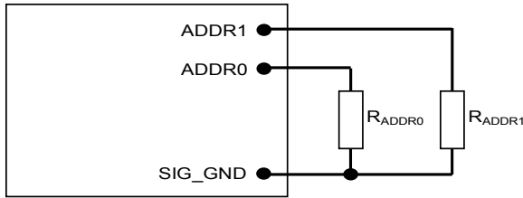
Figure 23. Circuit showing connection of resistors used to set the PMBus address of the module.
