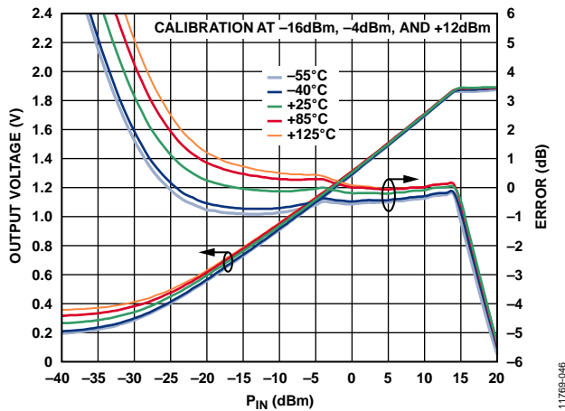
Figure 46. 2.14 GHz V_{RMS} and Log Conformance Error at +25°C, -40°C, -55°C, +85°C, and +125°C
