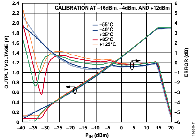
Figure 47. 2.14 GHz V_{RMS} and Log Conformance Error for Second Device at +25°C, -40°C, -55°C, +85°C, and +125°C
