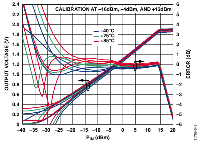
Figure 48. 2.14 GHz V_{RMS} and Log Conformance +25°C, -40°C, and +85°C for Multiple Devices
