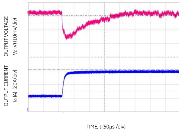
Figure 10. Transient Response to Dynamic Load Change from 25% to 75% at 12Vin, C O = 30x 47µF + 11x 1000µF, R TUNE = 3.74kΩ
